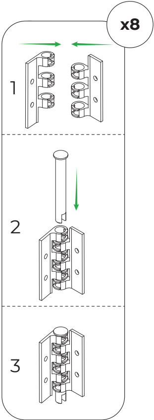
Hinge assembly
